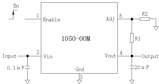
可调电压输出连接图 V_{OUT} = 1.240 \times [1 + (R1/R2)]
